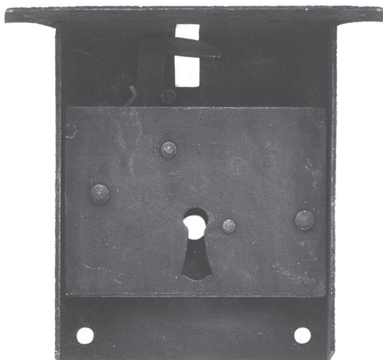
FPSH8/50-22A Lock for Chest Axis 50 mm ( 1.97 in )
